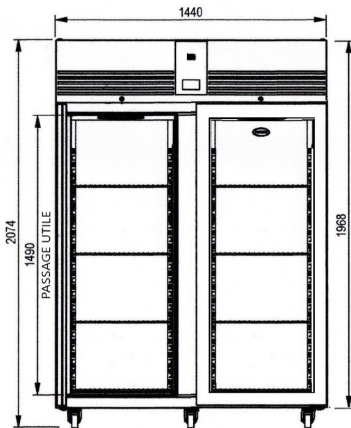
FACADE
